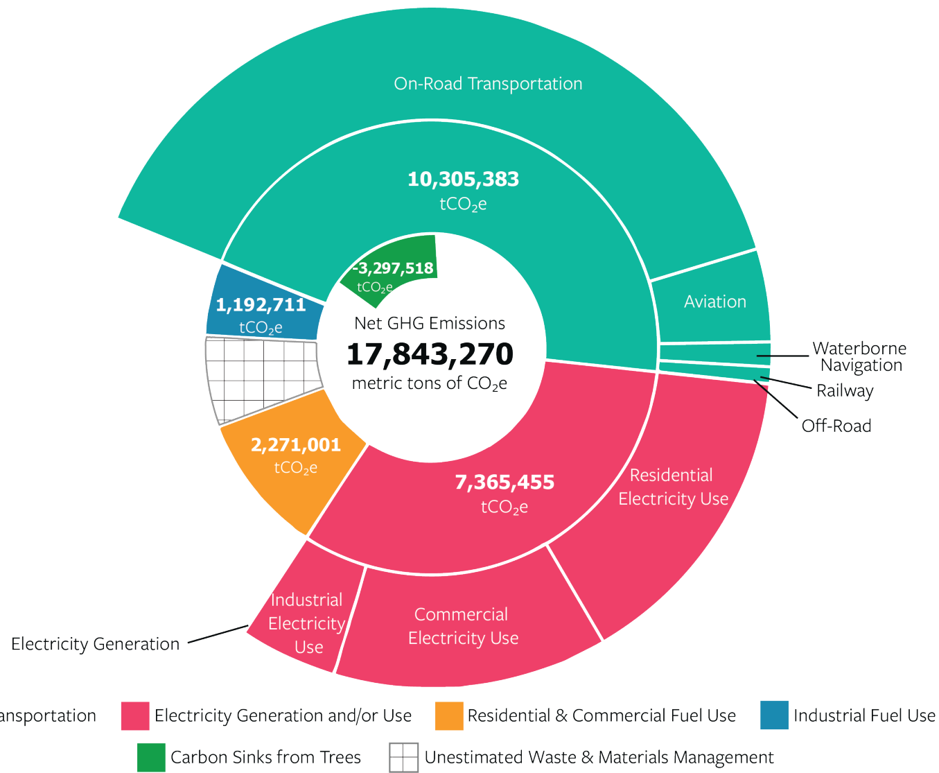
Figure 5. Simplified 2019 MSA-Wide GHG Emissions Estimates (metric tons of CO 2 e)
