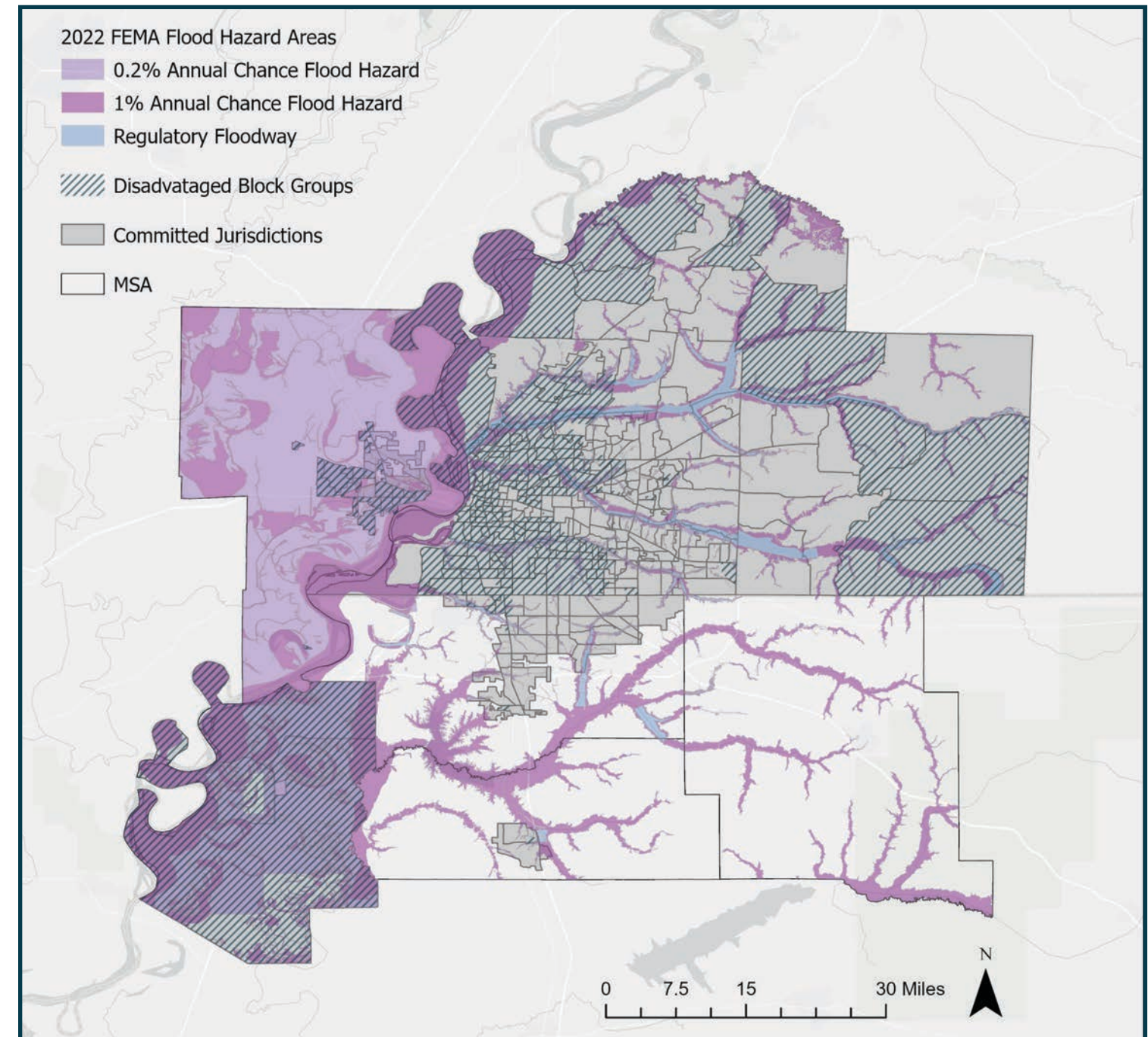
Figure 13. Flood Hazard Areas in the Memphis MSA
